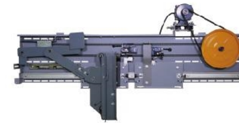
·MR-MVY-211 Center Opening Two Panel Operator (Car Frame Installation)
