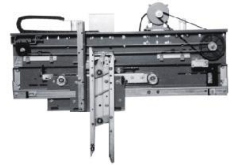
·MR-131-52B Side Opening VVVF Door Operator (Car Top Installation)
