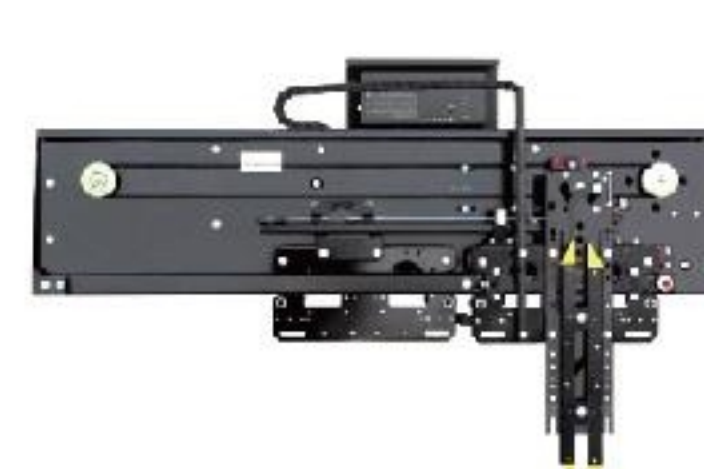
·MR-OSCAR-12/L-R Two Panels VVVF Telescopic Opening Car Door Operator
