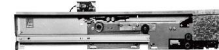
·MR-161-51 Side Opening Landing Door Mechanism
