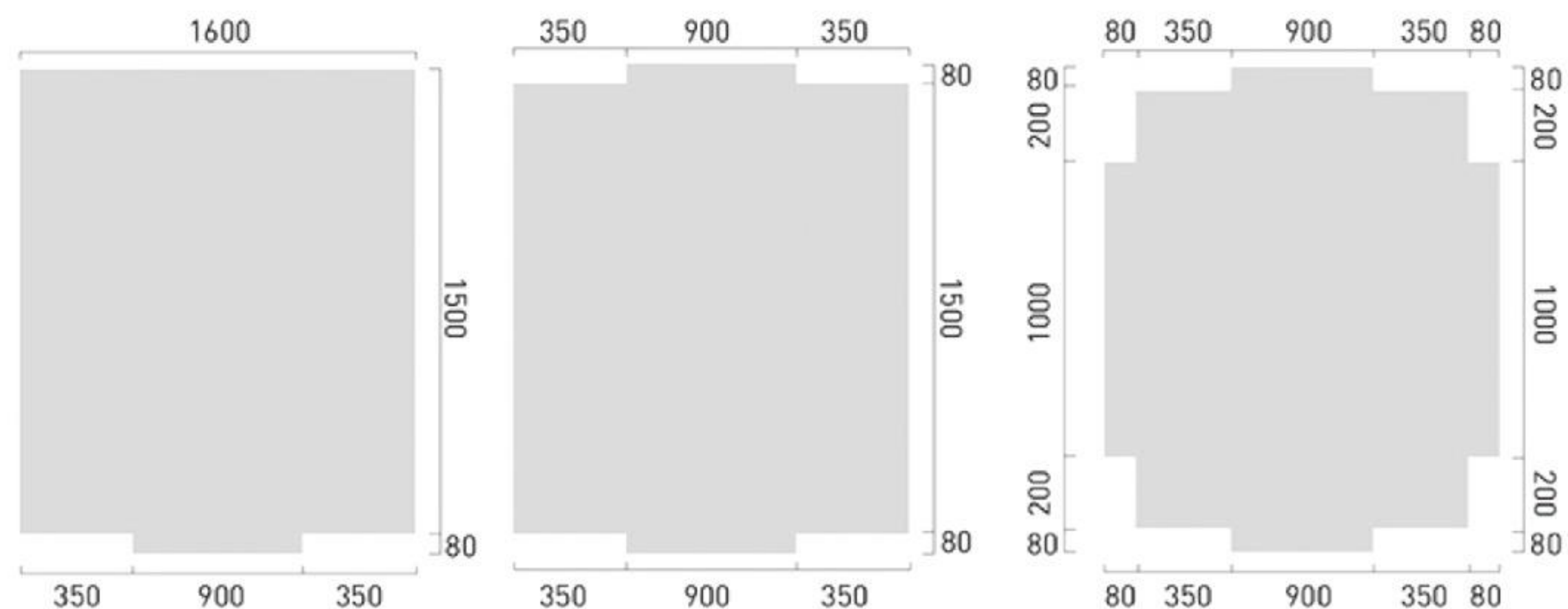
Standard elevator
