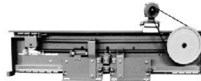
·MR-131-06A Center Opening VVVF Door Operator (Straight Beam Mounting)
