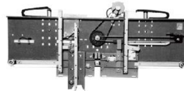
·MR-131-50-1A Center Opening VVVF Door Operator (Straight Beam Mounting)
