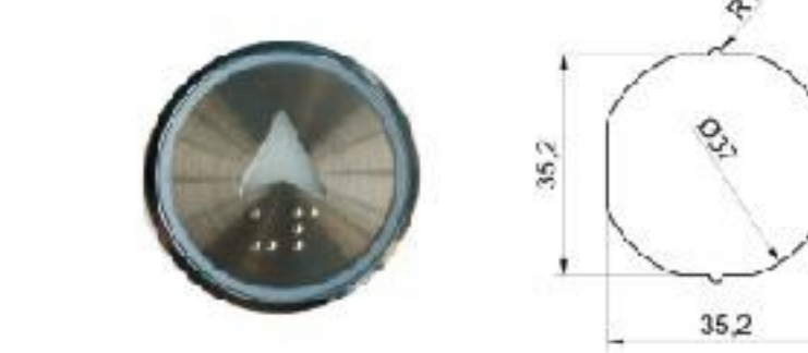
MR-EPB313B-C
