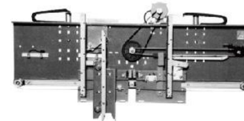
·MR-131-50-1B Center Opening VVVF Door Operator (Car Top Installation)
