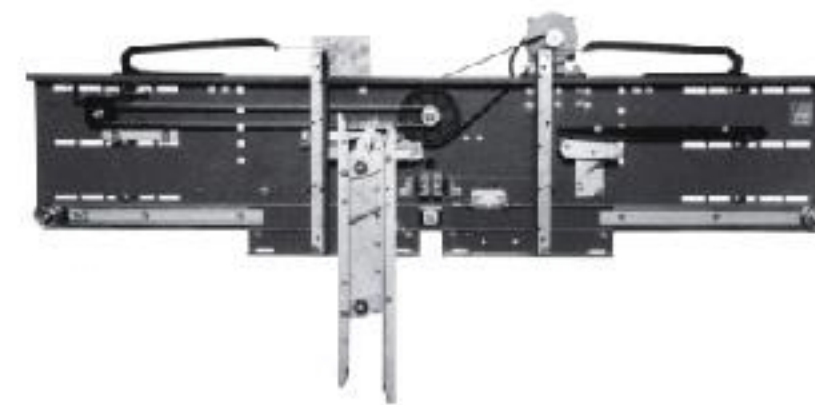
·MR-131-50B Center Opening VVVF Door Operator (Car Top Installation)
