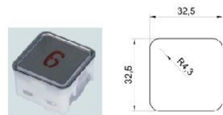
MR-EPB270
