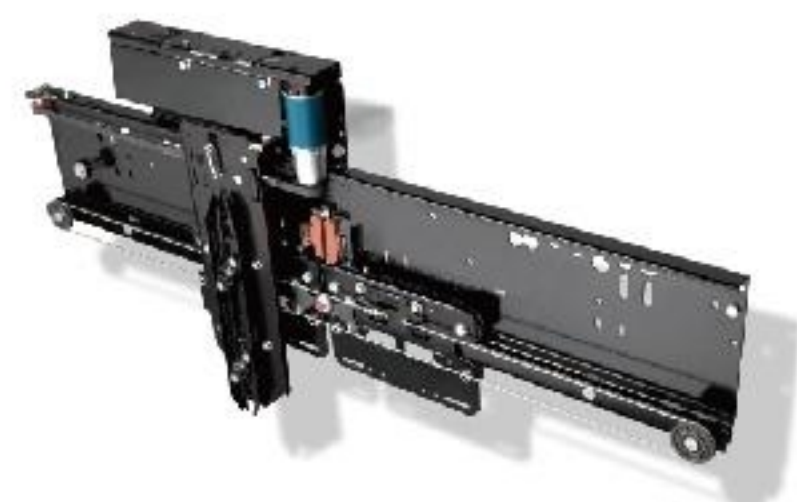
·MR-ECO-02/C Two Panels Center Opening Car Door Operator
