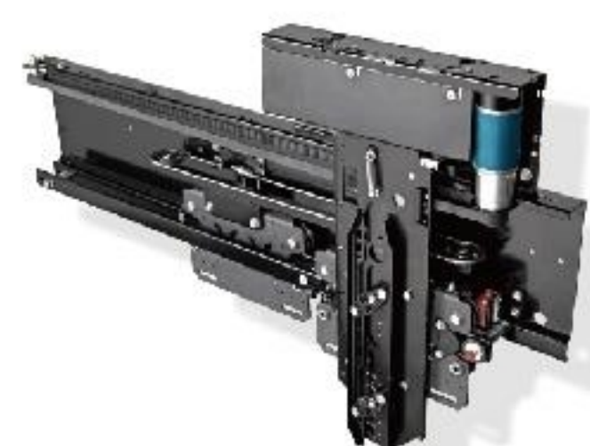
·MR-ECO-12/R-L Two Panels Telescopic Opening Car Door Operator
