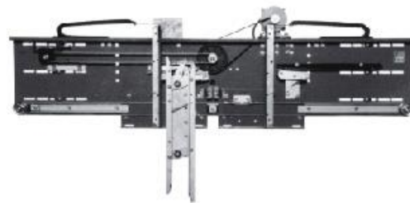
·MR-131-50A Center Opening VVVF Door Operator (Straight Beam Mounting)
